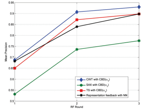
Figure 10: Comparison of representation feedback with item diversity
